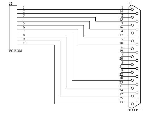
BACKGROUND DEBUGGER
