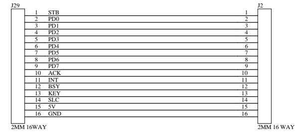
DIGITAL COLOUR CAMERA TO EYEBOT CAMERA PORT
