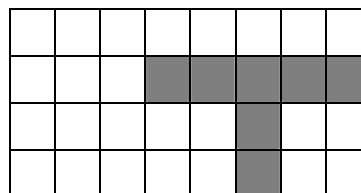
Text
