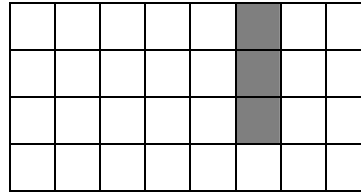
“AND”
