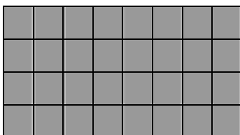
Graphic
